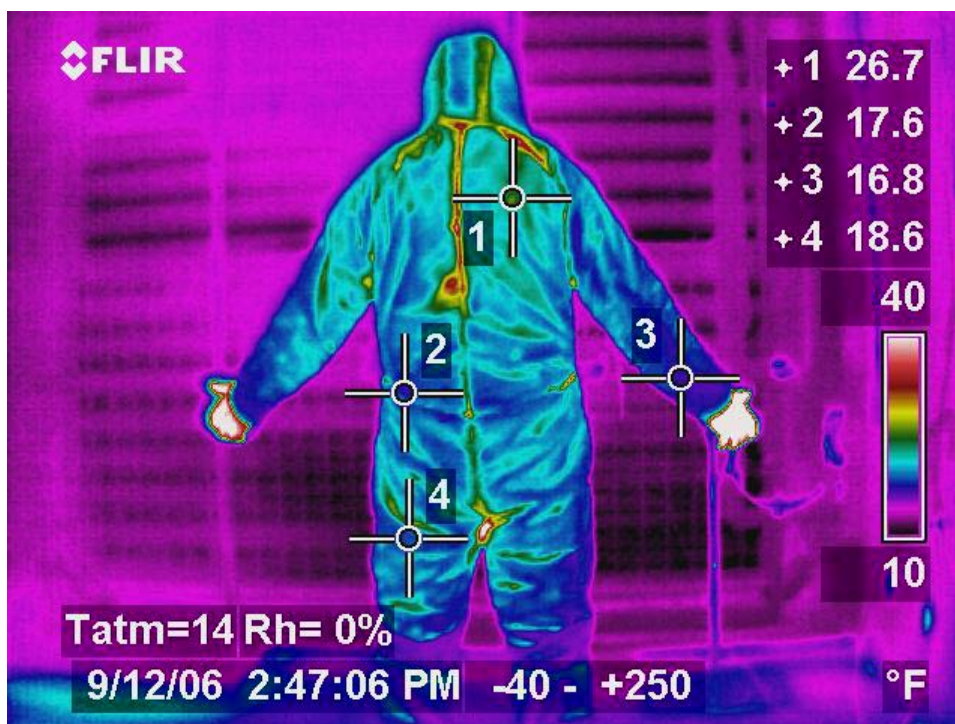
Figure 6. Back view of aerogel garment. Typical surface temperatures 17-27°F.
