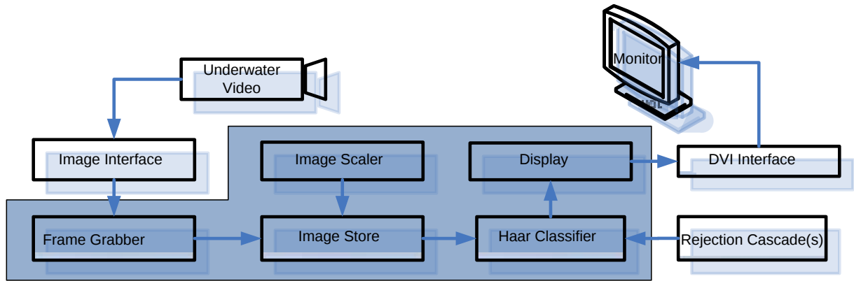
Figure 5. FPGA framework.
