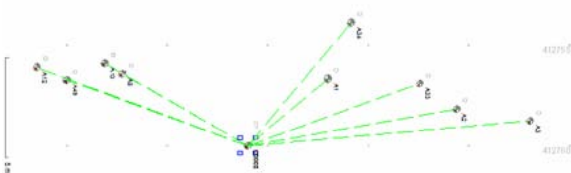
Figure 1. Preliminary survey of Butrint wrecksite. Courtesy of Dr. Jeff Royal, RPMNF.
