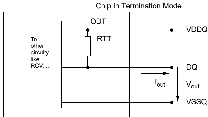
Figure 73 — On Die Termination
