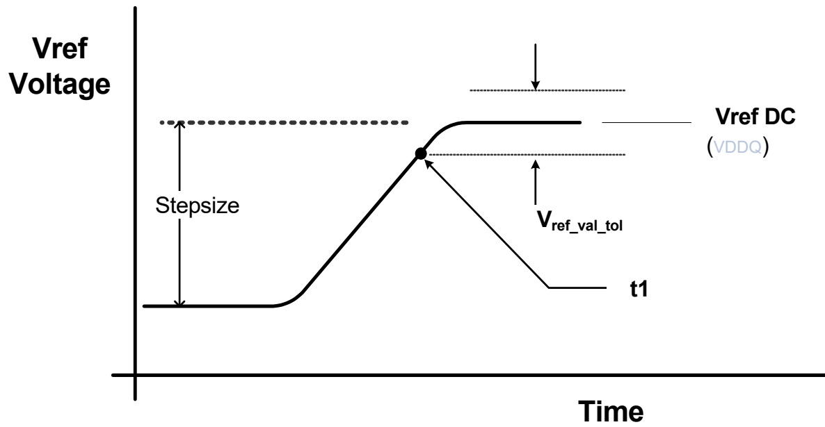
Figure 40 — Vref step single stepsize increment case.
