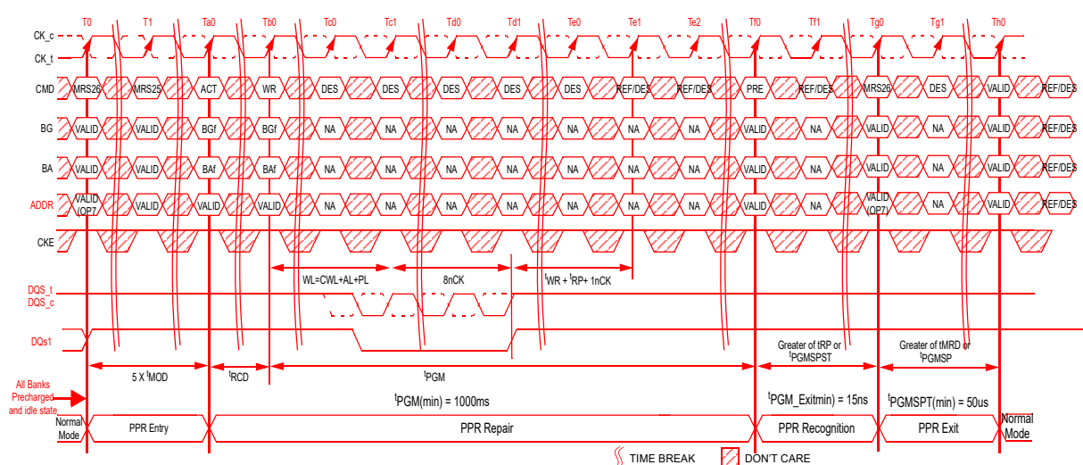
Figure 52 — hPPR Fail Row Repair
