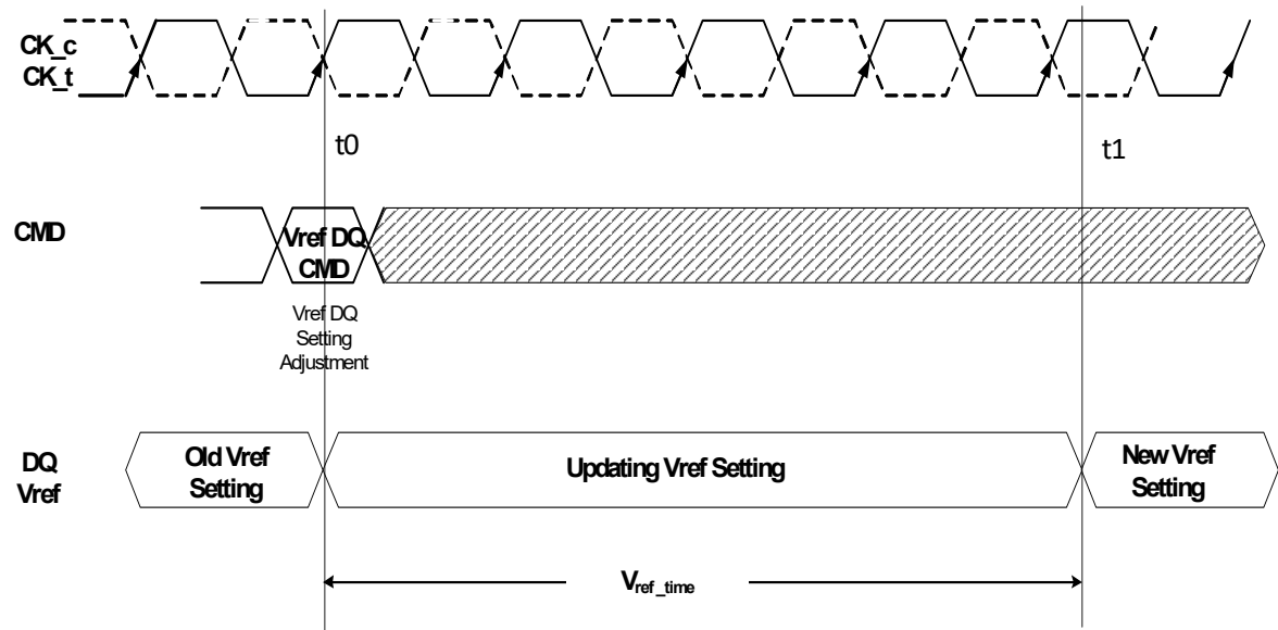
Figure 46 — Vref_time timing diagram
