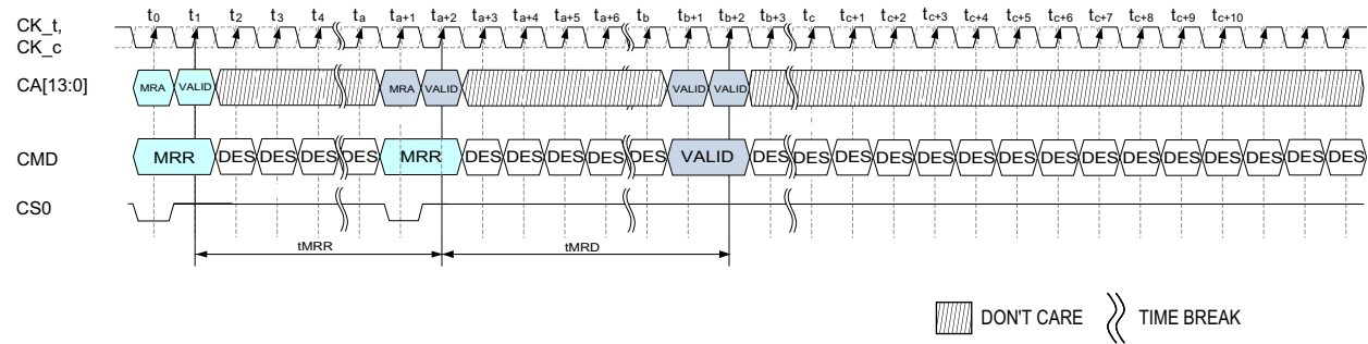
Figure 5 — Mode Register Read Timing
