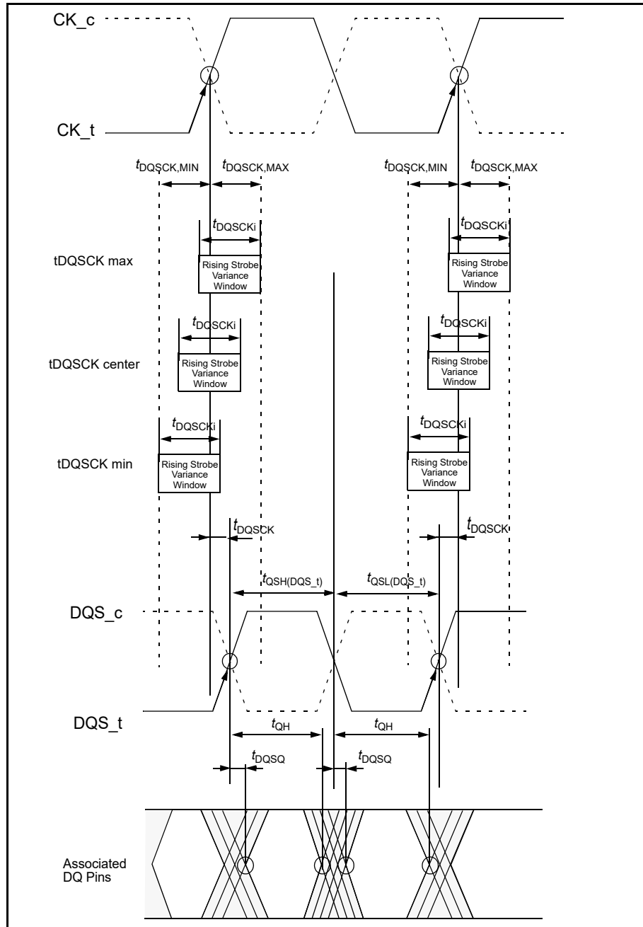
Figure 7 — TDQSCK Timing Definition
