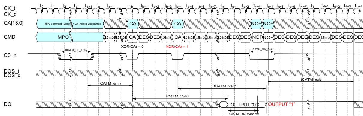
Figure 28 — Timing Diagram for CA Training Mode
