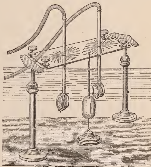
Fig. 3. Apparatus of M. Bjercknes for tracing automatically the lines of hydro-dynamic force.
