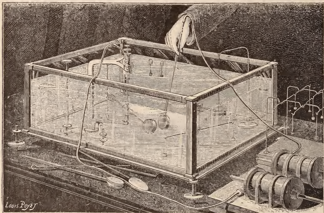
Fig. 1. Apparatus of M. Bjerknæs at the Electrical Exposition.
