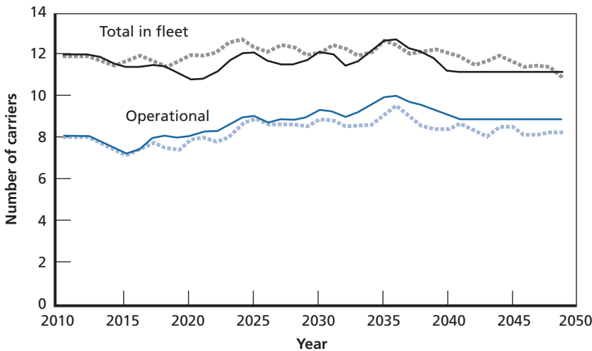
Figure S.2 A Build-New Plan Sustains at Least as Many Operational Ships and Almost as Many Total as the Navy’s Current Plan (Reference Case)
