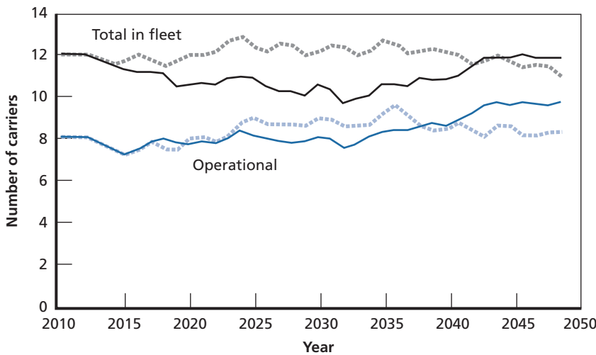
Figure 2.16 Ship Life Sustained by 30-Month Build-New Interval and 30-Year Unrefueled Life Span
