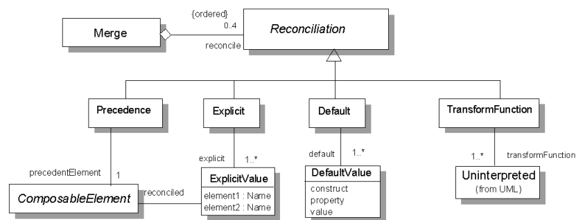
Figure 71: Reconciliation Specification
