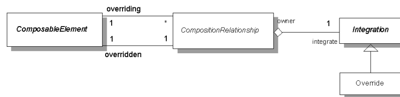
Figure 43: Override Integration
