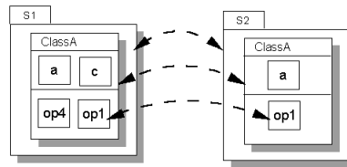
Figure 21: Explicit Correspondence
