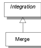
Figure 70: Merge Integration
