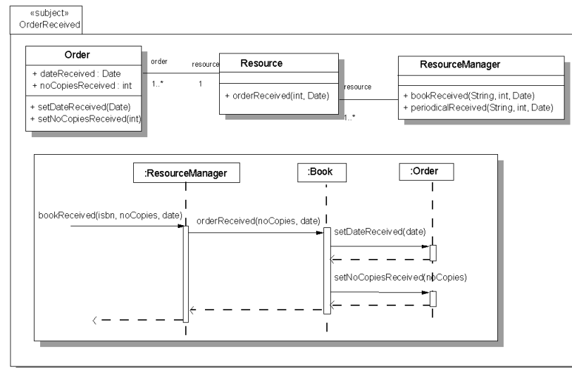
Figure 137: Order Received
