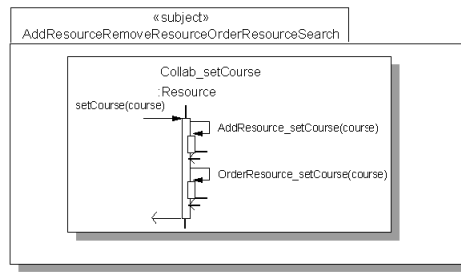
Figure 130: Generated Interaction
