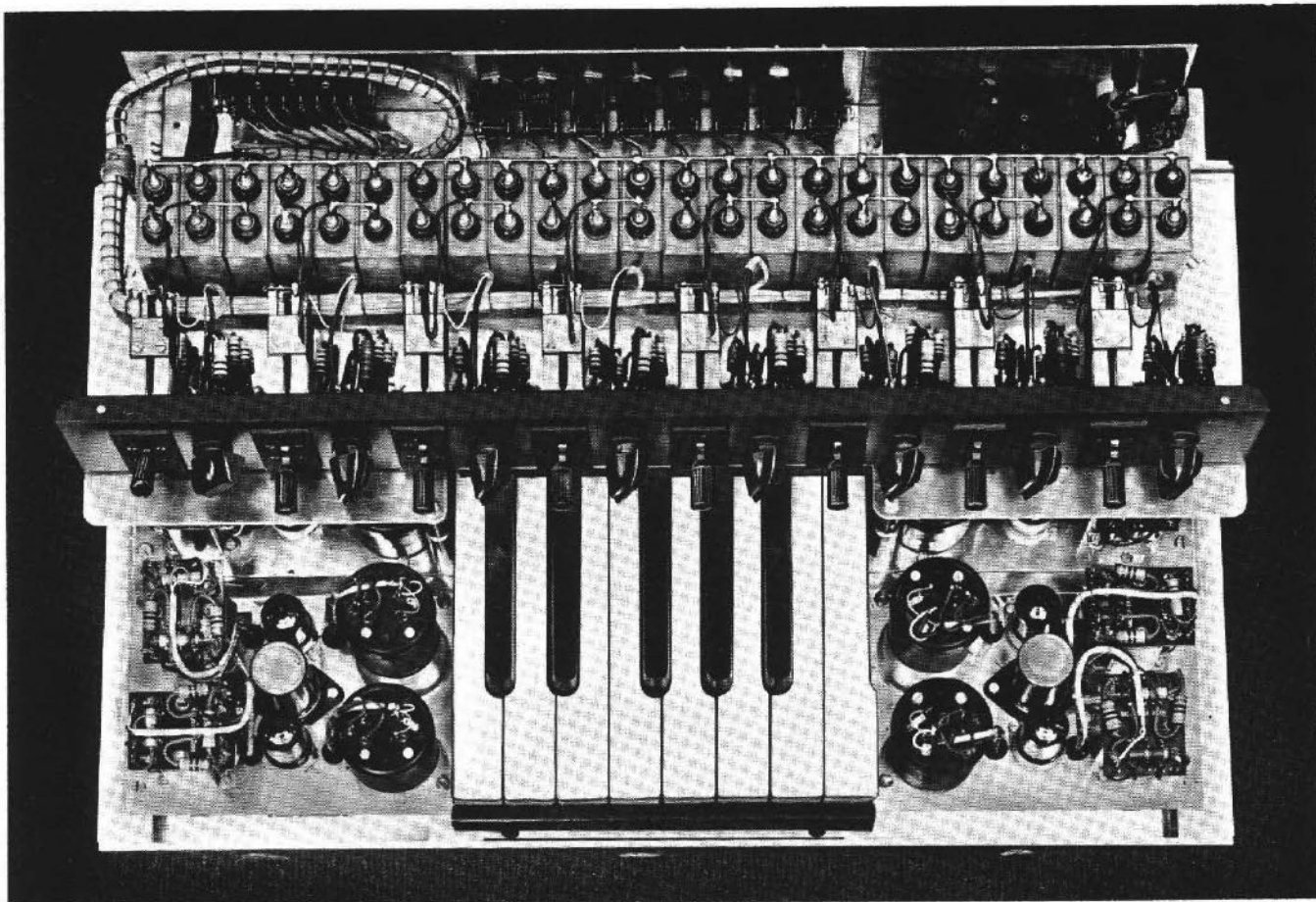
Fig. 7 — Photograph of keying unit, cover removed.
