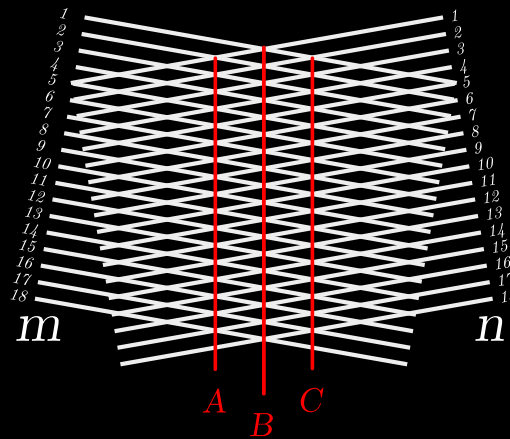
FIGURE 1. Moiré Lines
