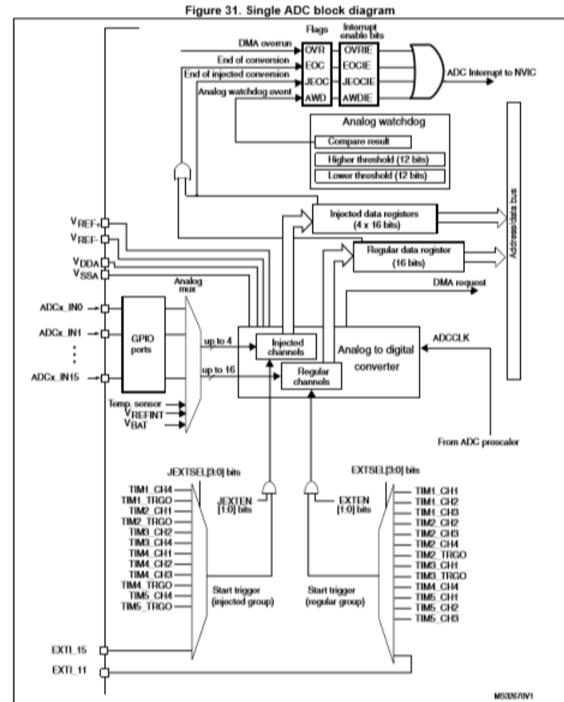
Figure 31 shows a single ADC block diagram and Table 40 gives the ADC pin description.
