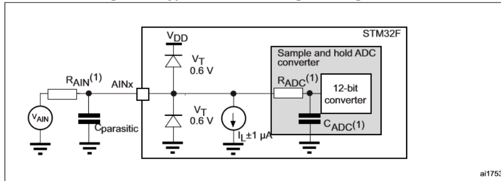
Figure 41. Typical connection diagram using the ADC
